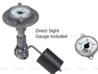
Dash Mounted Gauge
